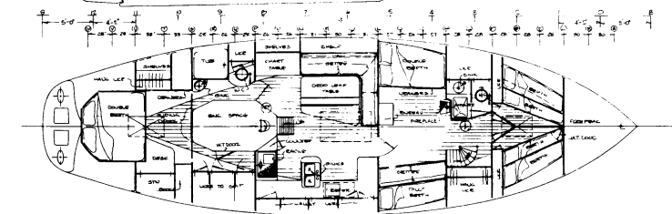
60' Topsail Schooner
