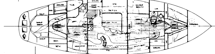
60' Ketch Harambee
