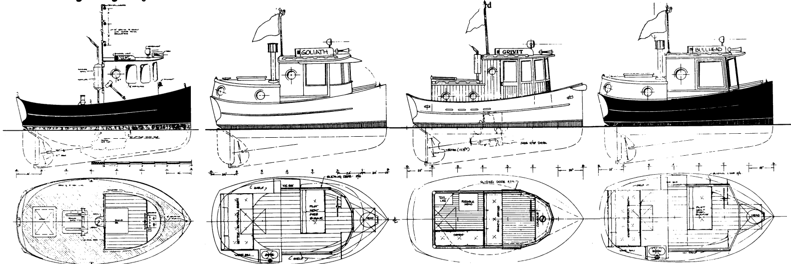
14' Tugboat 14' x 13' x 7' x 3'
