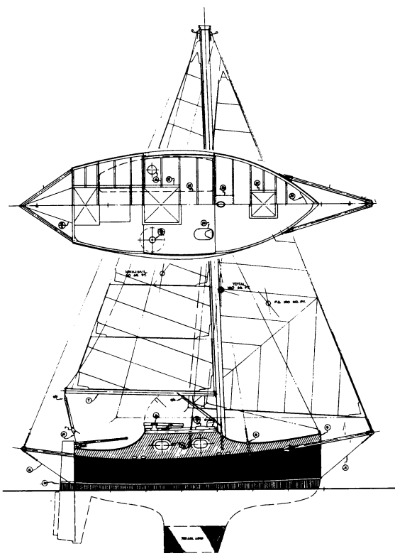
14' Cruiser Happy 13'-10" x 18'-8" x 6'-3" x 3'-7"
