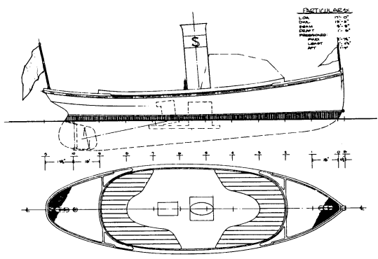
17' Fantail Steam Launch Myf 17 x 15'-6" x 5'-3" x 1'-8"
