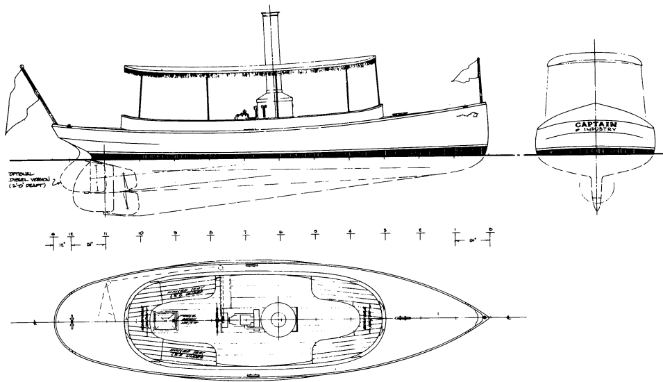
25' Fantail Steam Launch Beverley 25' x 22'-6" x 7' x 3'-3"
